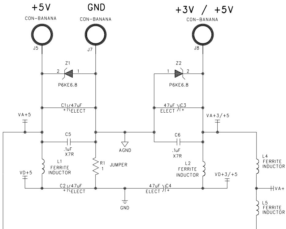
Figure 7. Power Supply
