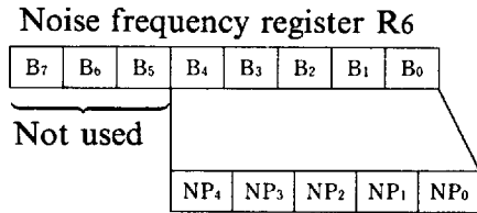
5 bit noise frequency setting value (NP)
